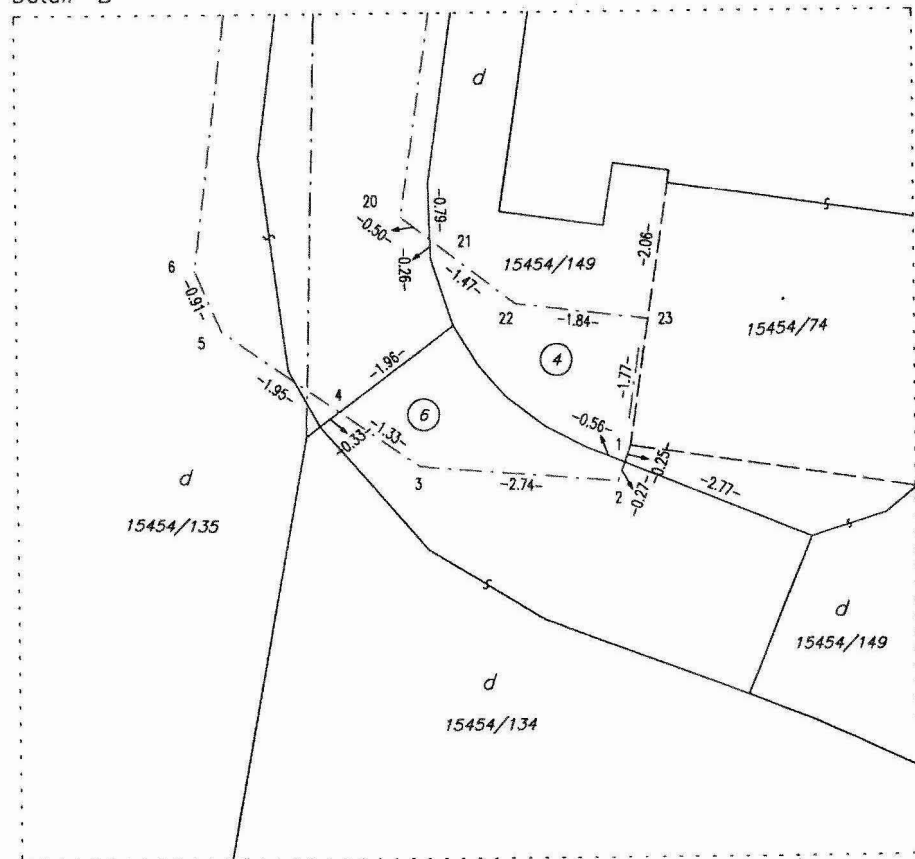
Detail "B"
