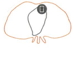
Figure 5 - T310d 5GHz Elevation Antenna Patterns
