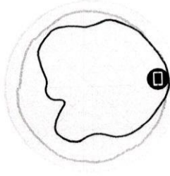
Figure 3 - T310d 5GHz Azimuth Antenna Patterns
