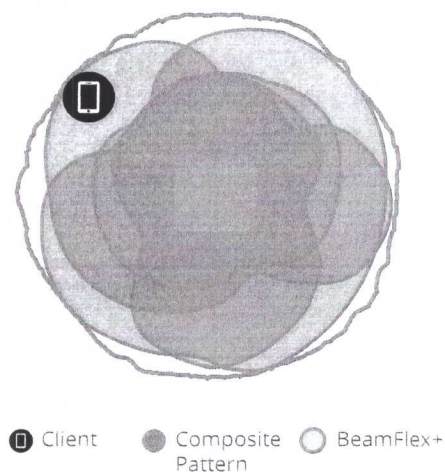
Figure 5. 5GHz Elevation Antenna Patterns
