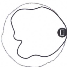
Figure 3. 5GHz Azimuth Antenna Patterns
