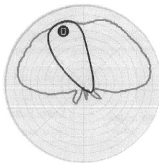
Figure 4. 2.4GHz Elevation Antenna Patterns
