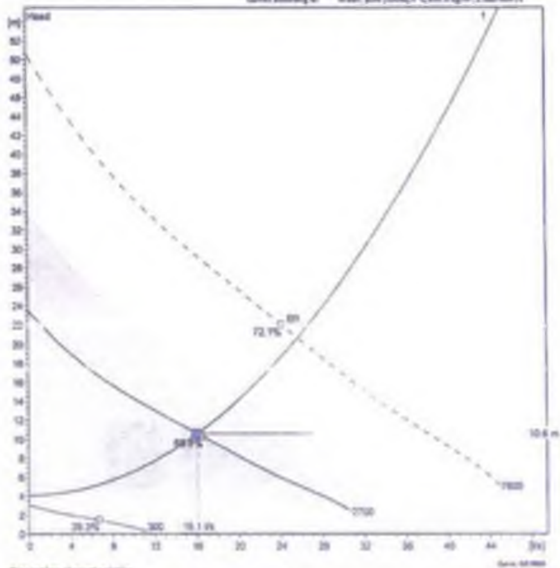
Operating characteristics
