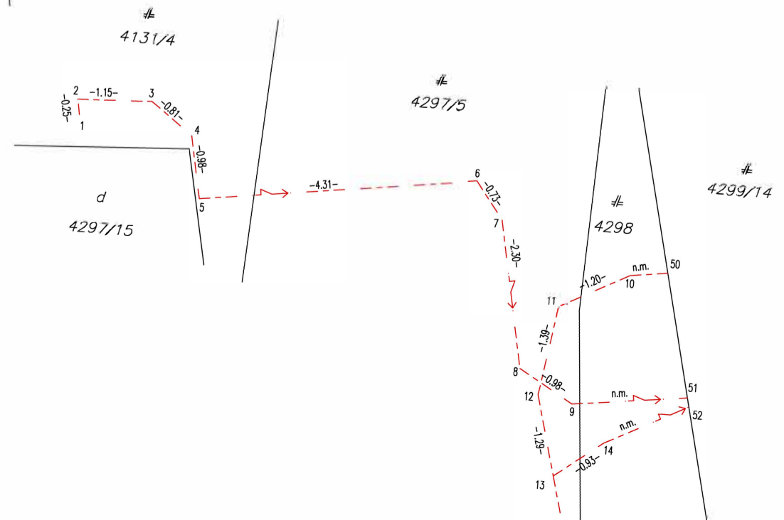
Detail "A"
