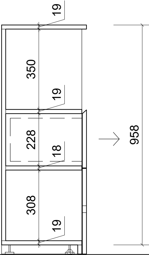
REZ 1:10
