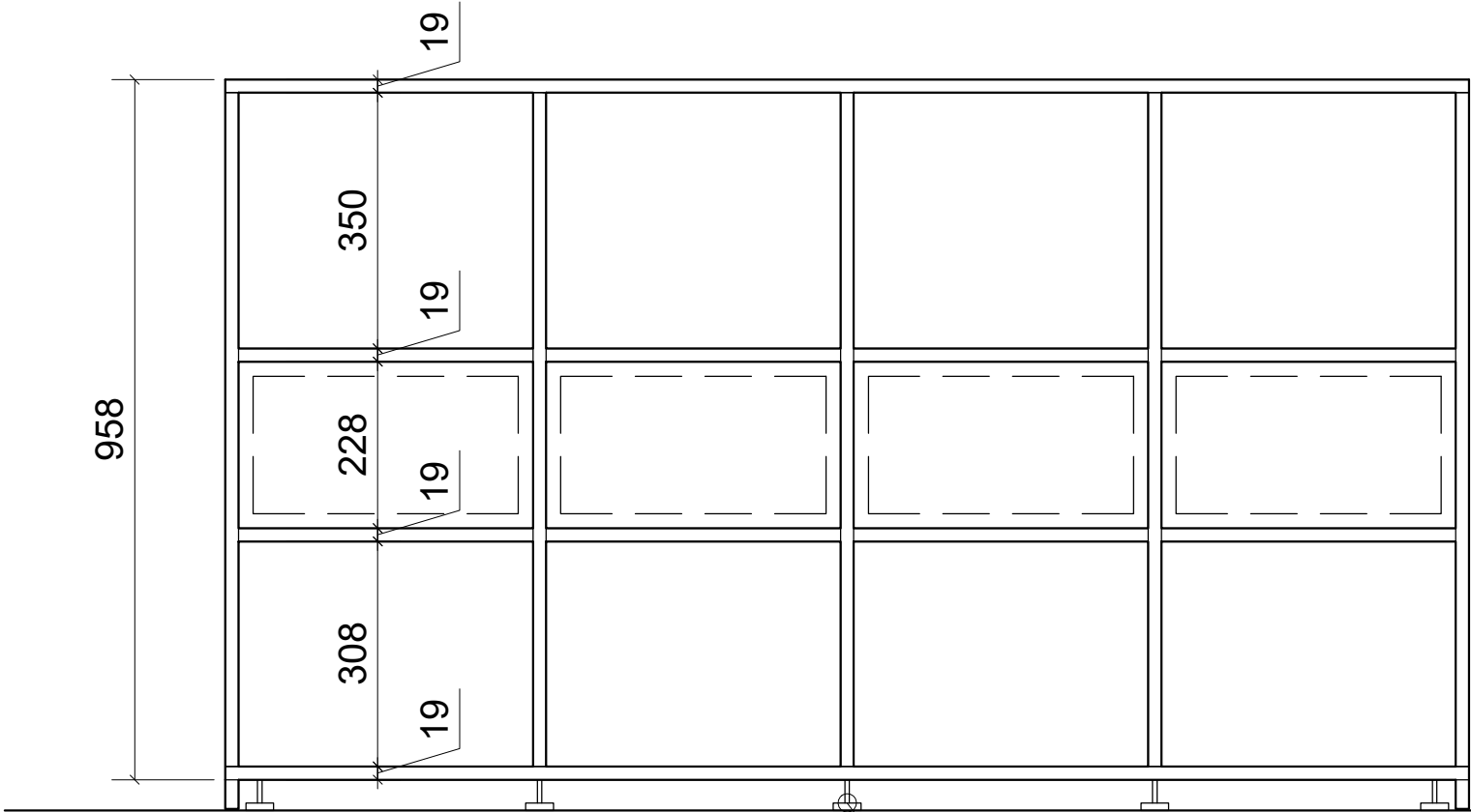
REZ 1:10
