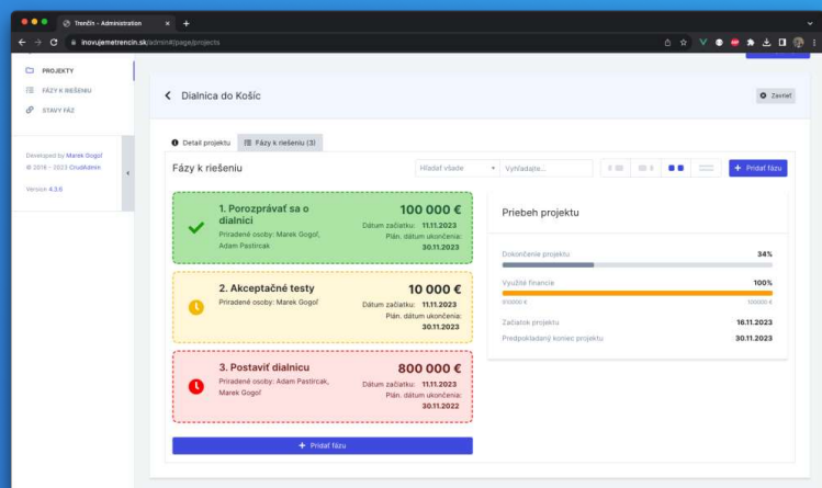
Admin panel
