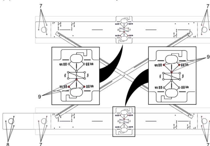
Figure 6 - Drilling positions
